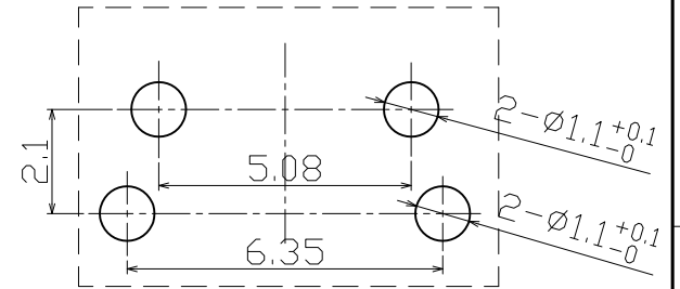
P.C.B mounting hole detail
