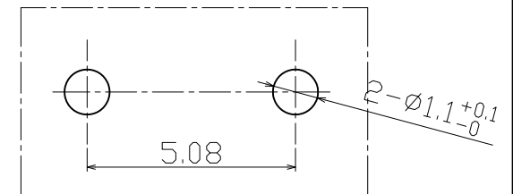
P.C.B mounting hole detail
